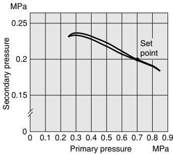
● HRS110-□-TF
