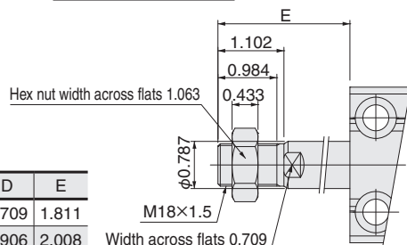
-B: Male thread specifications
