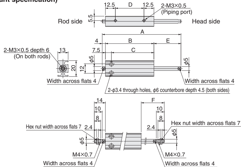
-B: Male thread specifications
