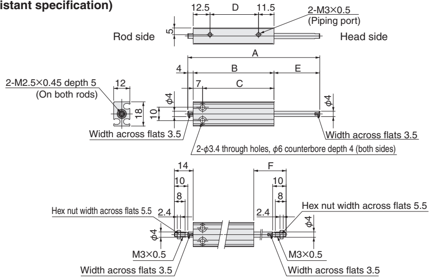
-B: Male thread specifications
