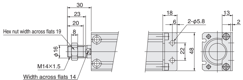
-B: Male thread specifications
