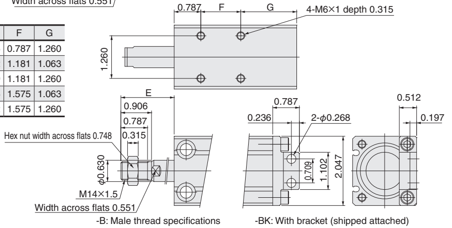
-B: Male thread specifications
